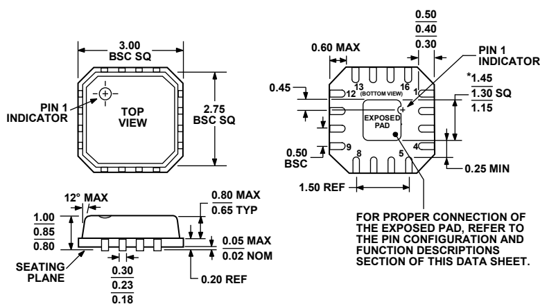
Figure 46. 16-Lead Lead Frame Chip Scale Package [LFCSP_VQ] 3 mm × 3 mm Body, Very Thin Quad (CP-16-2) Dimensions shown in millimeters
